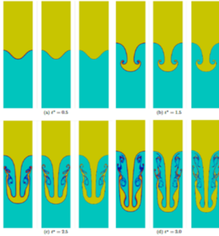
Figure 5 CLS field contour for Rayleigh-Taylor instability problem at different timestamps with meshes \{25 \times 100, 50 \times 200, 100 \times 400\} , shown from left to right.
