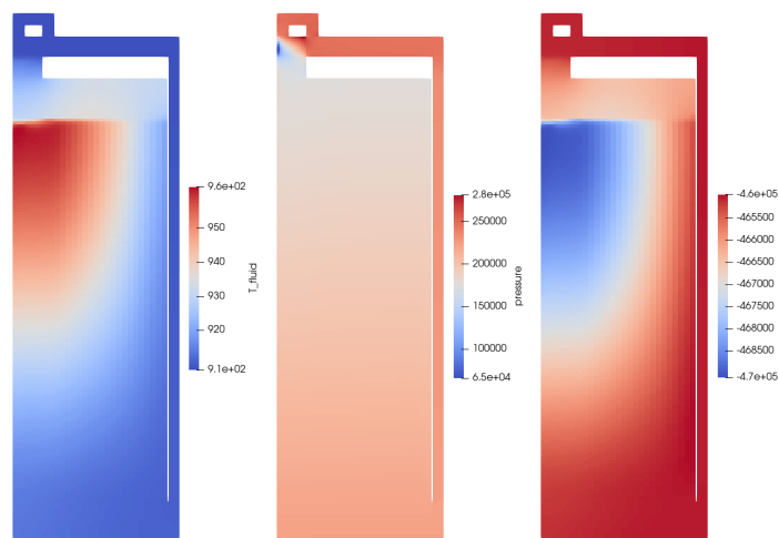
Figure 4 Thermochemically important fields within MSRE at steady-state operation predicted by the coupled MSR simulator: (a) temperature [K], (b) pressure [Pa], (c) chemical potential of fluoride ( F^- ) [J/mol].
