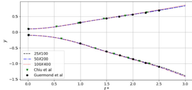
Figure 6 Interface location along the domain center and boundary with different mesh compared with results from Guermond et al [3] and Chiu et al [4]
